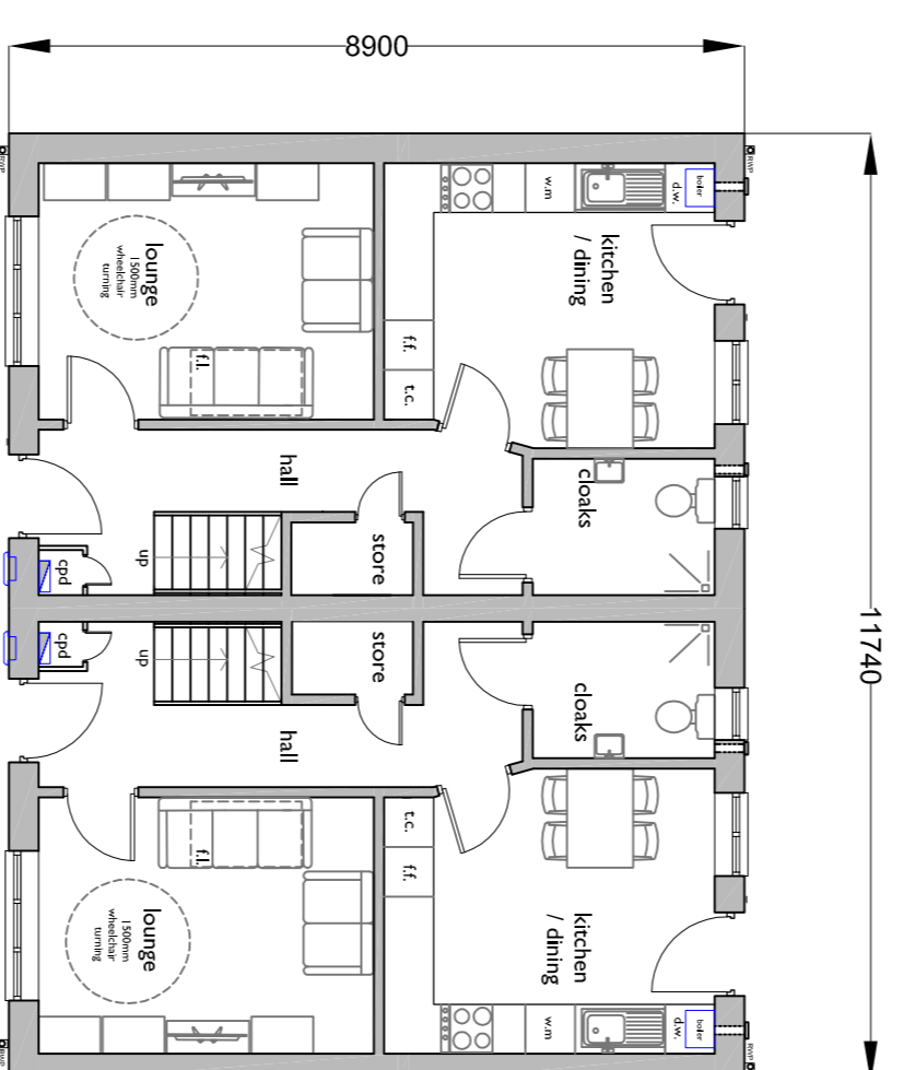
Cynllun Lawr Gwaelod Arfaethedig 1:100 Proposed Ground Floor Plan 1:100
