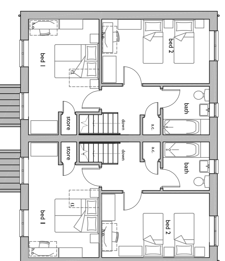
Cynllun Lawr Cyniat Arfaethedig 1:100 Proposed First Floor Plan 1:100
