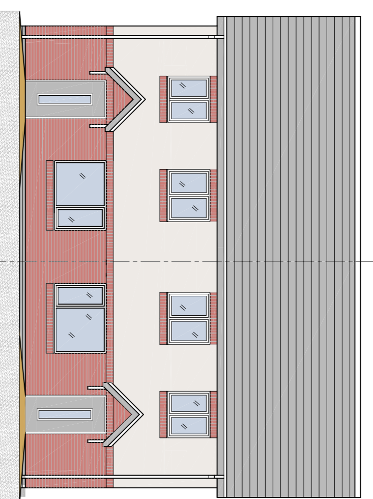
Edrychiad Blaen Arfaethedig 1:100 Proposed Front Elevation 1:100
