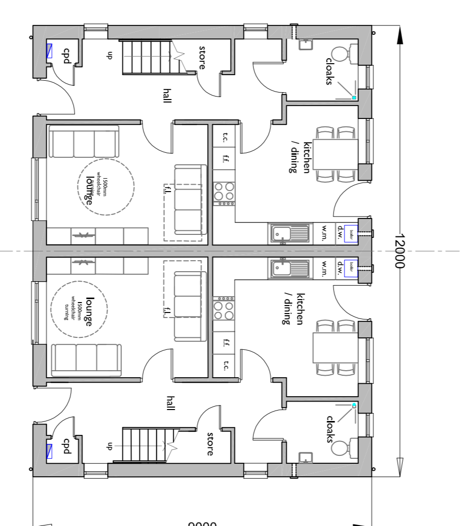
Cynllun Llauer Gwaedol Arfaethedig 1:100 Proposed Ground Floor Plan 1:100
