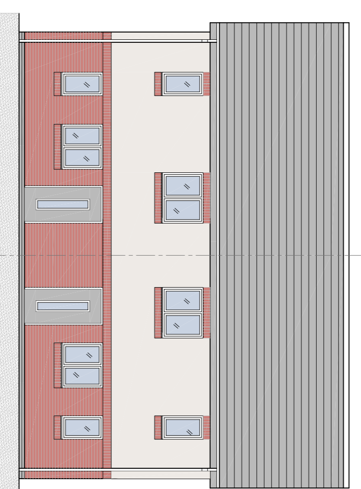
Edrychiad Cefn Arfaethedig 1:100 Proposed Rear Elevation 1:100
