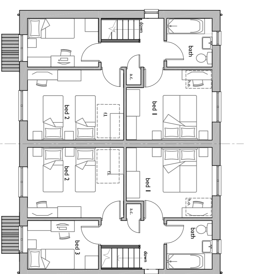
Cynllun Llauer Cyntaf Arfaethedig 1:100 Proposed First Floor Plan 1:100
