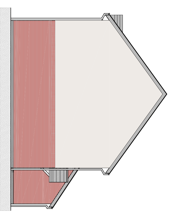
Edrychiad Ochr Arfaethedig 1:100 Proposed Side Elevation 1:100
