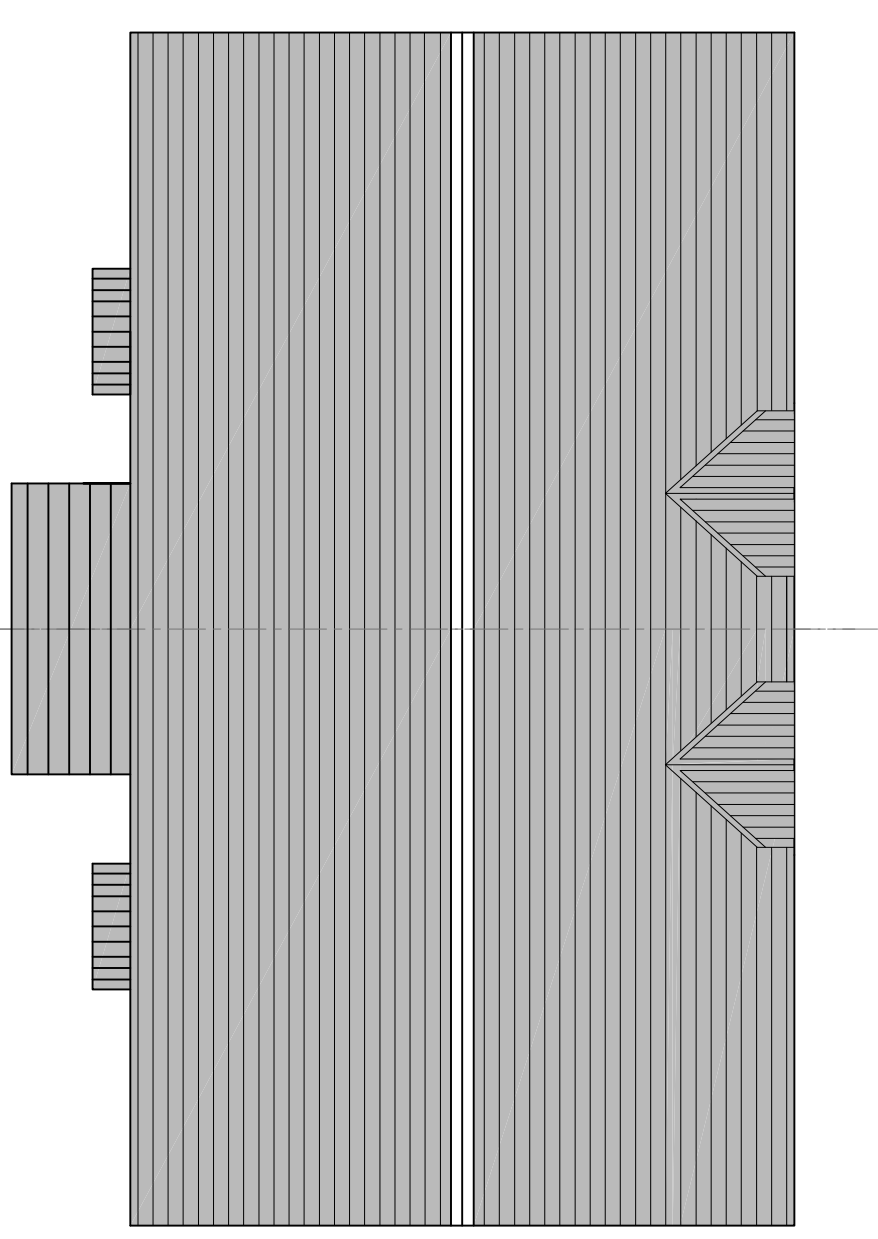
Cynllun To Arfaethedig 1:100 Proposed Roof Plan 1:100
