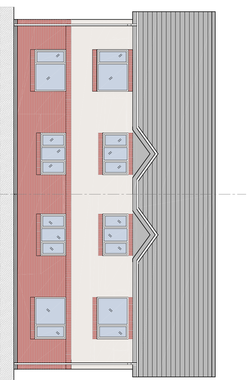
Edrychiad Cefn Arfaethedig 1:100 Proposed Rear Elevation 1:100
