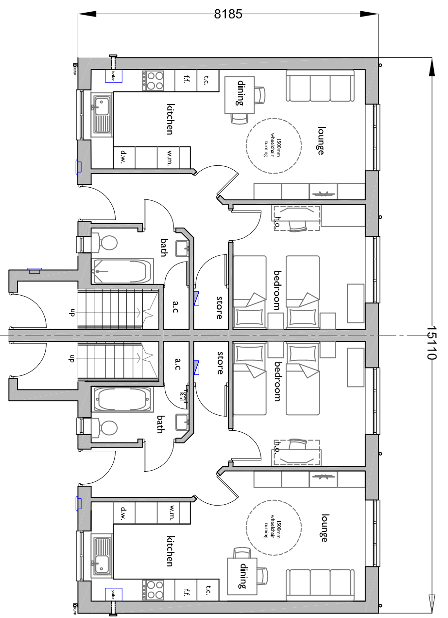
Cynllun Llwr Gwaelod Arfaethedig 1:50 Proposed Ground Floor Plan 1:50
